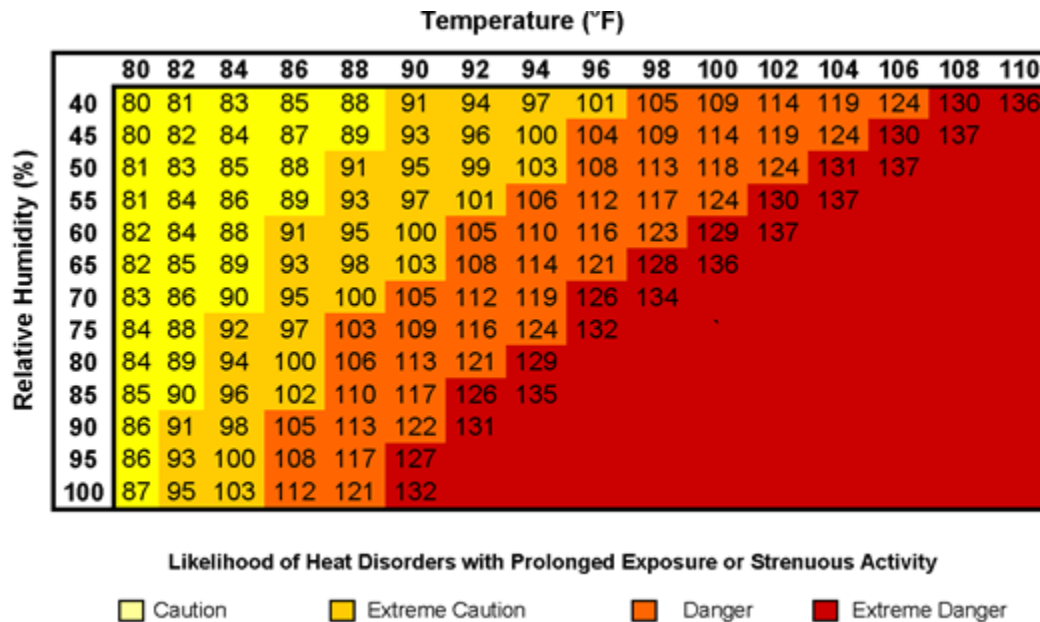
Figure 3.7.11-8 Heat Index
