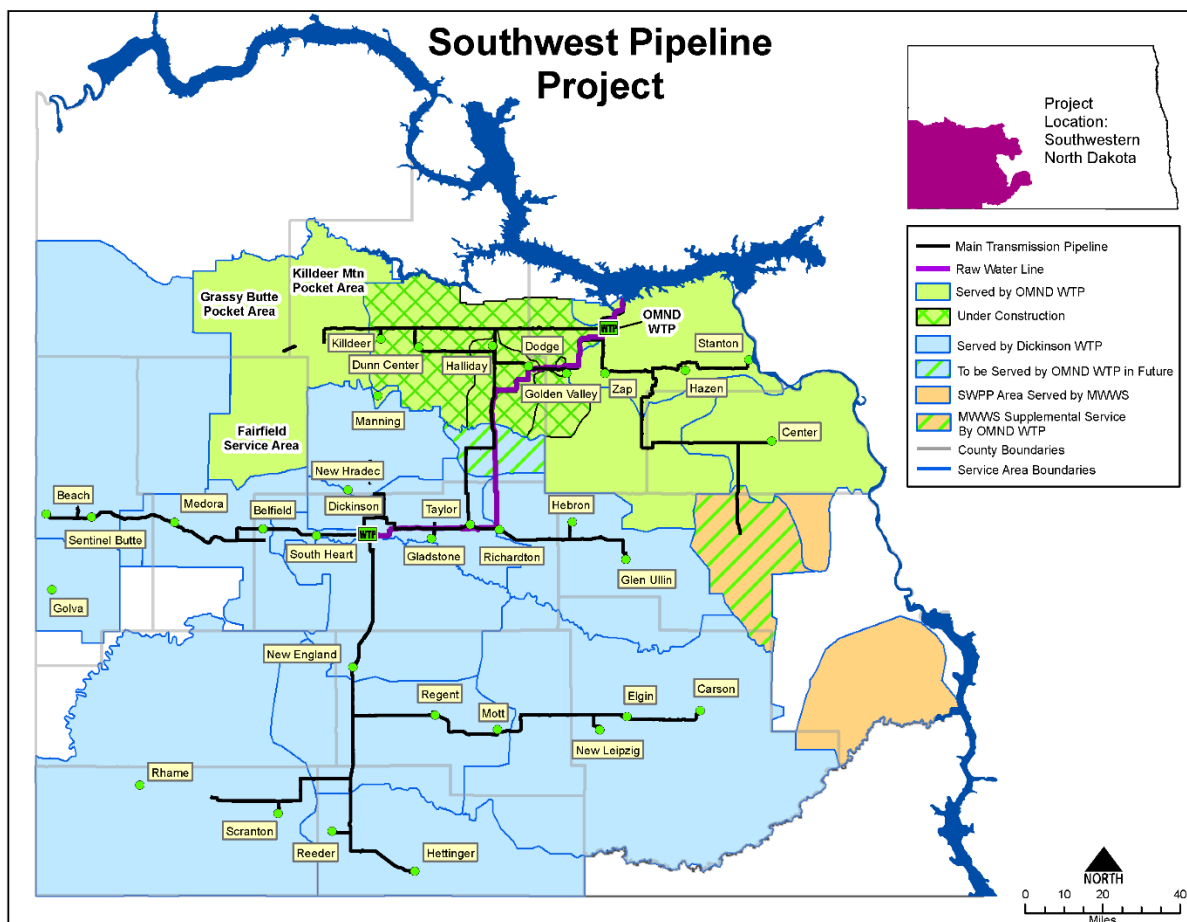
Figure 7.4.3-4: Southwest Pipeline Project
