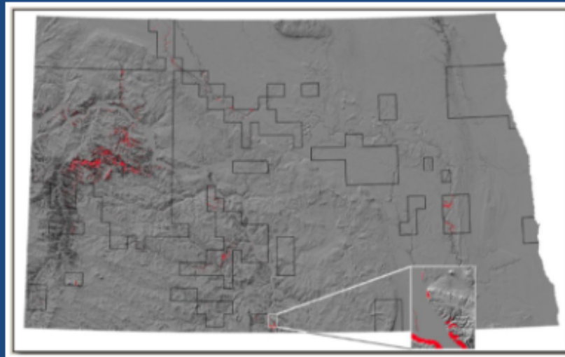
Identified Landslides in North Dakota by the North Dakota Geological Survey (NDGS, 2017)
