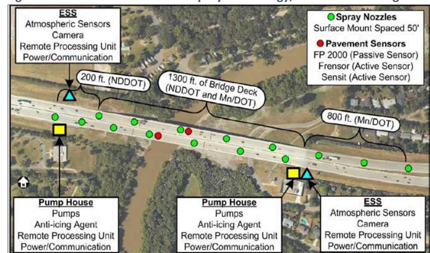
Figure 4.15-44: Fixed Automated Spray Technology, on Red River Bridge
