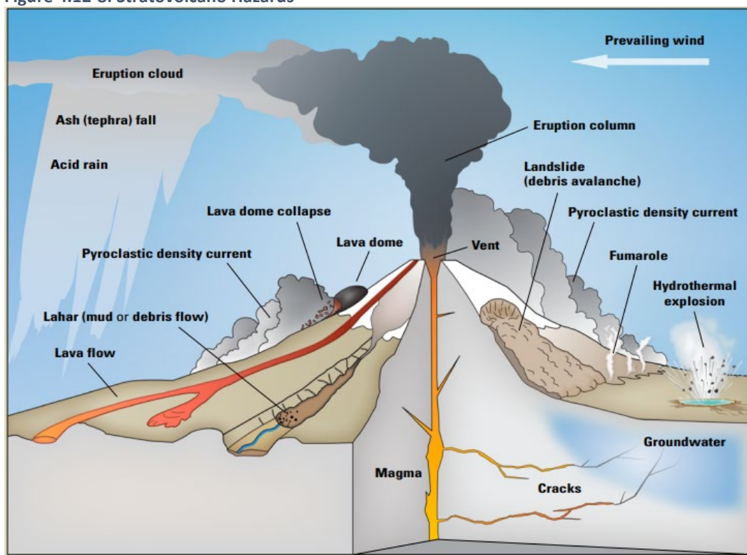
Figure 4.12-8: Stratovolcano Hazards
