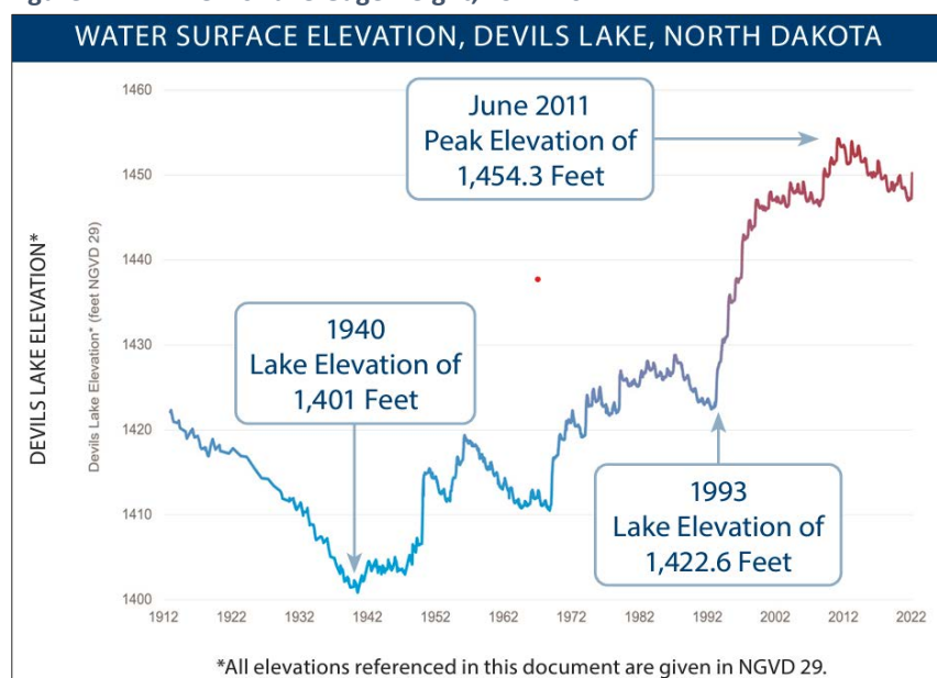
Figure 4.1-22: Devils Lake Gage Height, 1912-2022
