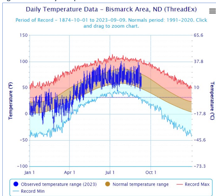
Figure 2.62: Daily Temperature in Bismarck
