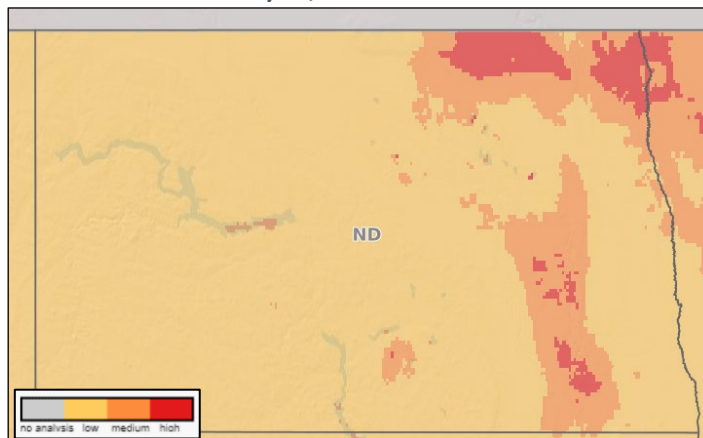
Figure 4.7-46: Penn State University's Fusarium Risk Tool Output for North Dakota on July 26, 2023
