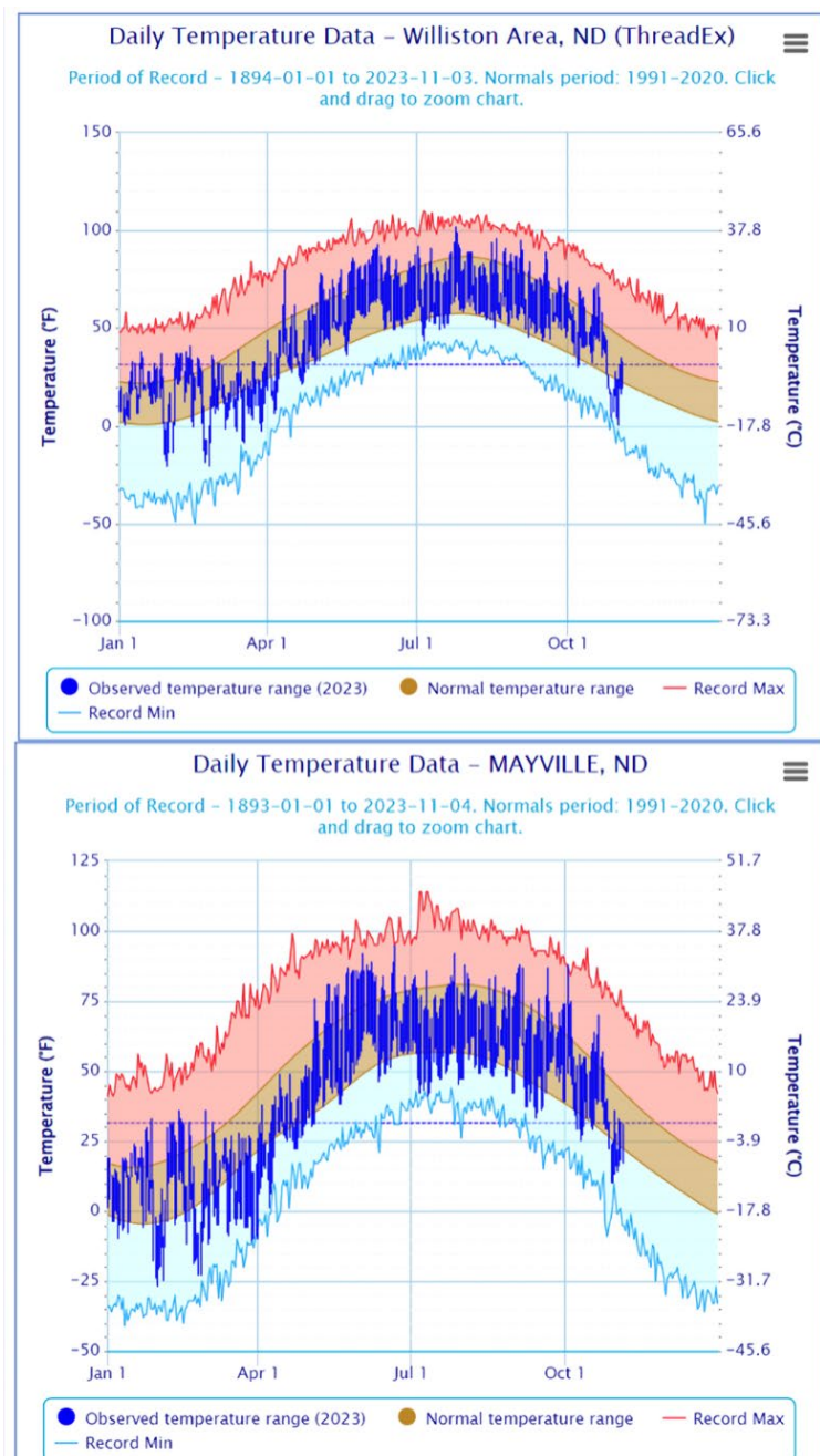
Figure 3-1: Daily Temperature for Williston and Mayville, ND
