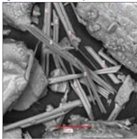
Figure 4.12-6: Erionite Crystals
