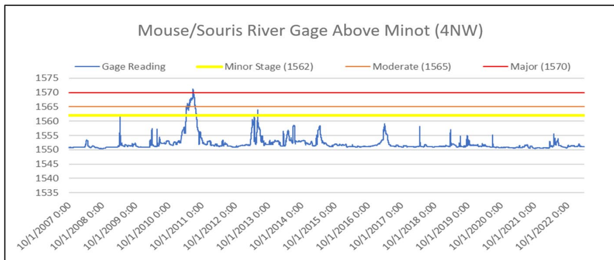
Figure 4.1-21: Mouse/Souris River Gage at Minot, WY2008-2023
